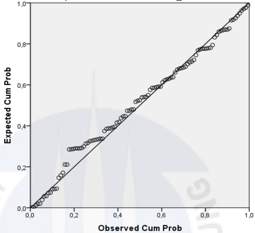
Normal P-P Plot of Regression Standardized Residual Dependent Variable: TOTAL_GG
