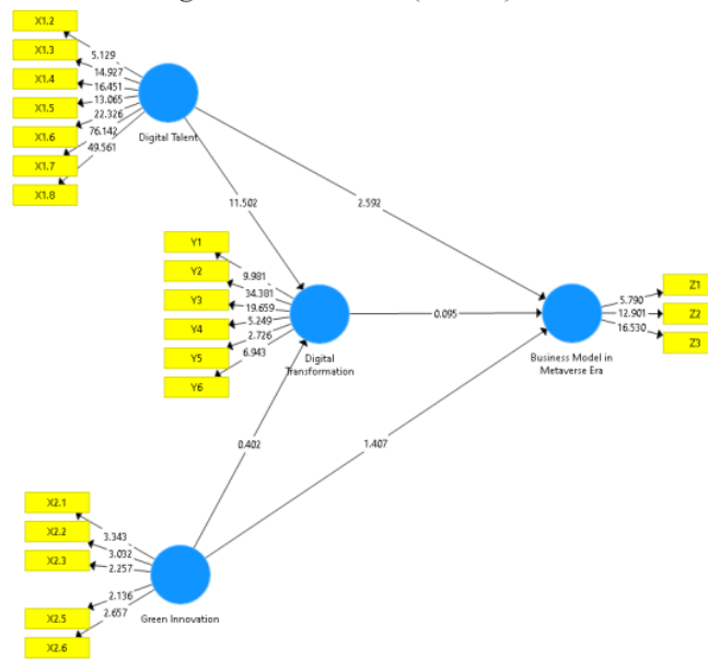
Figure 7. Final Model (z-value)
