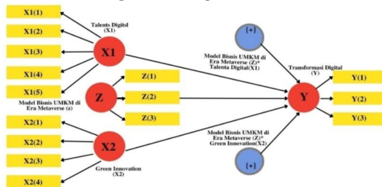
Figure 3. Path diagram with PLS
