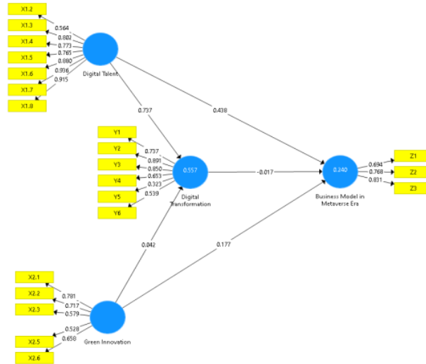
Figure 6. Final Model (Loading factors)
