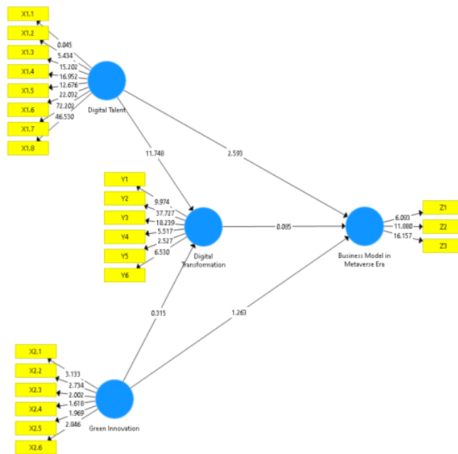
Figure 5. Initial model (z-values)
