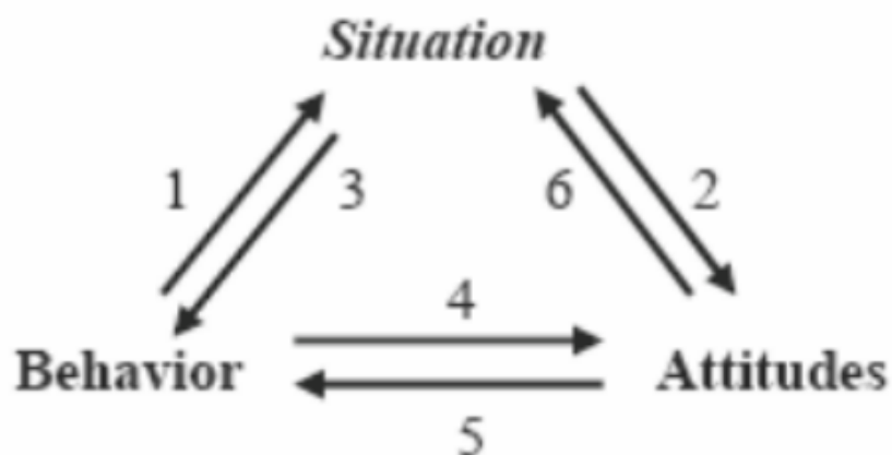
Gambar 1. Model Konflik Mitchell
