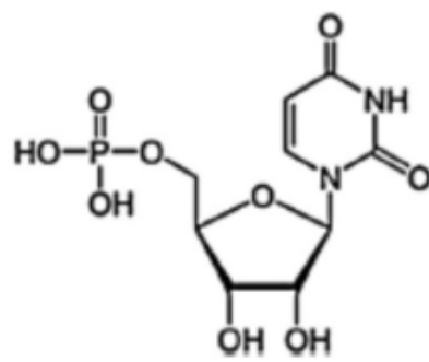
Uracil 5' monophosphate nucleotide
