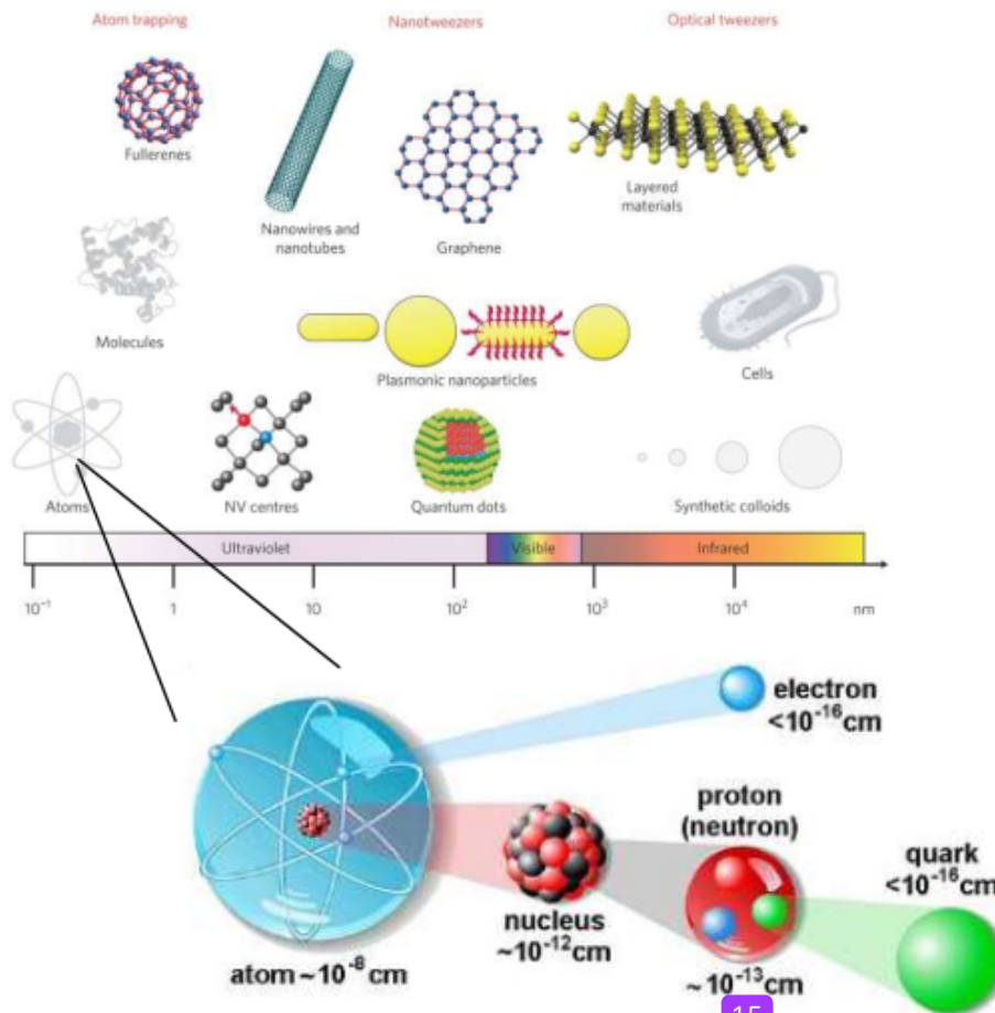
Gambar 46. Fundamental structure of an atom and the three size ranges of optical trapping. Objects of different sizes can be trapped within three main regimes (from left to right): atom trapping (a few ångstroms to a few nanometres), nanotweezers (a few nanometres to a few hundred nanometres) and optical tweezers (from a fraction of a micrometre up). The horizontal scale bar shows the average object size and the corresponding light wavelength. NV, nitrogen vacancy. Image of layered material reproduced from ref. 169, © 2011 NPG [112, 113] .
