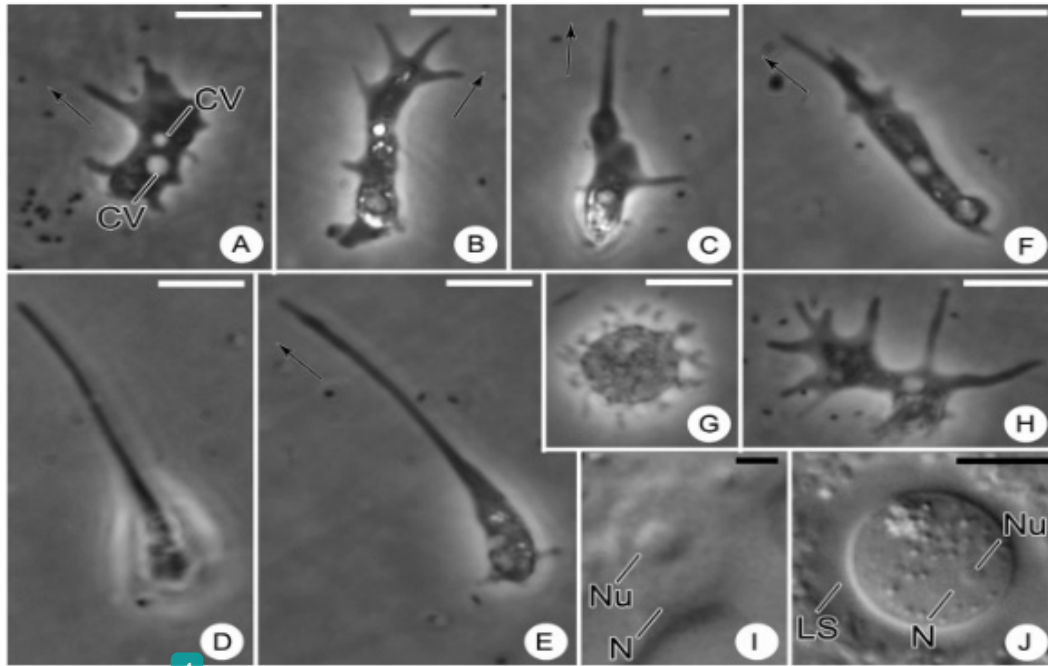
Gambar 23. Korotnevelva fosta n.sp. Light micrographs of living amoebae. (A-C) Locomotive forms. Arrows indicate the direction of movement. (D-F) Three consecutive stages of formation of long subpseudopodium. Arrows indicate the direction of movement. (D) An amoeba with "leading" subpseudopodium, which detached from the substratum and waving in the water. (E) The same cell with a subpseudopodium, which laid on the substratum. (F) The same cell with cytoplasmic cell body flowing into the subpseudopodium. (G) Stationary cell. (H) Non-directionally moving cell. (I) Cell compressed with a cover slip showing the nucleus. (J) A cyst compressed with a cover slip. Contractile vacuole (CV), nucleus (N), nucleolus (Nu), layer of scales (LS). Scale bars 10m (A-H), 1m (I), 5m (J) [52] .
