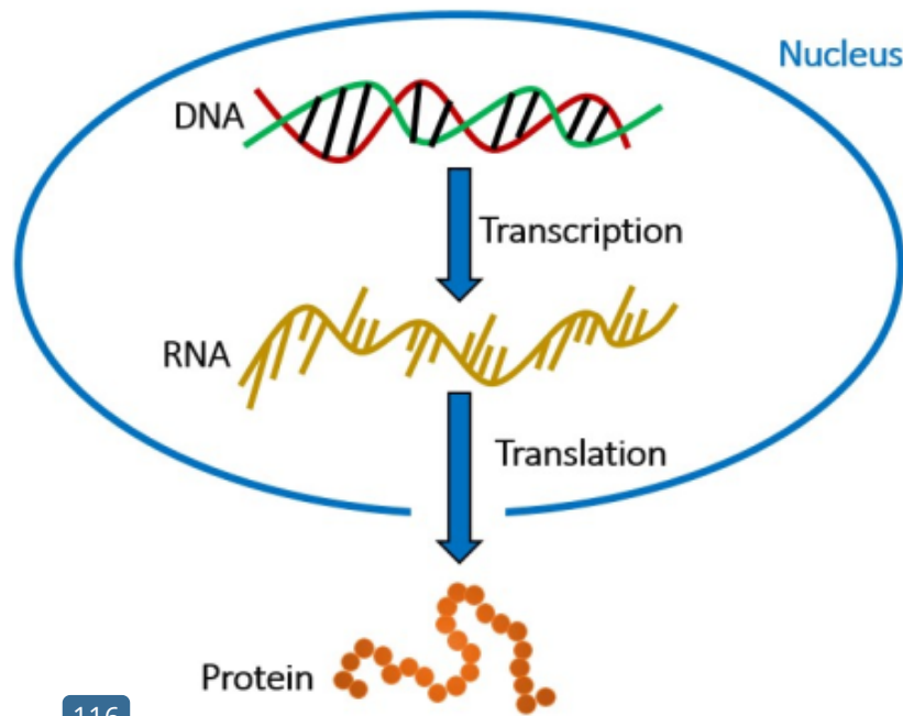
Gambar 42. 116 Overview of the central dogma 78 is the flow of genetic information inside a biological system. In order to make protein, a cell first transcribes genetic information from DNA onto a temporary template of RNA. Then each RNA translates a set of specific information for synthesis of a particular protein [101]
