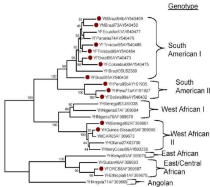
Gambar 44. Phylogenetic tree of yellow fever viruses with a G100S E protein mutation [108] .
