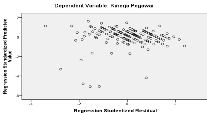
Scatterplot
