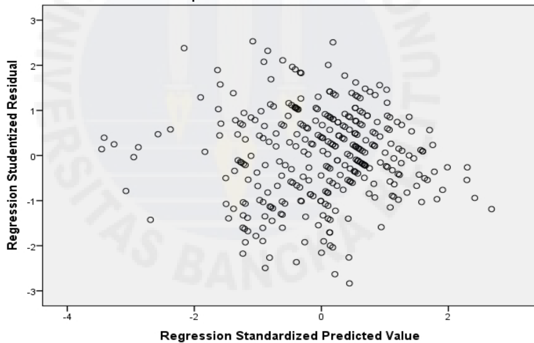
Scatterplot
