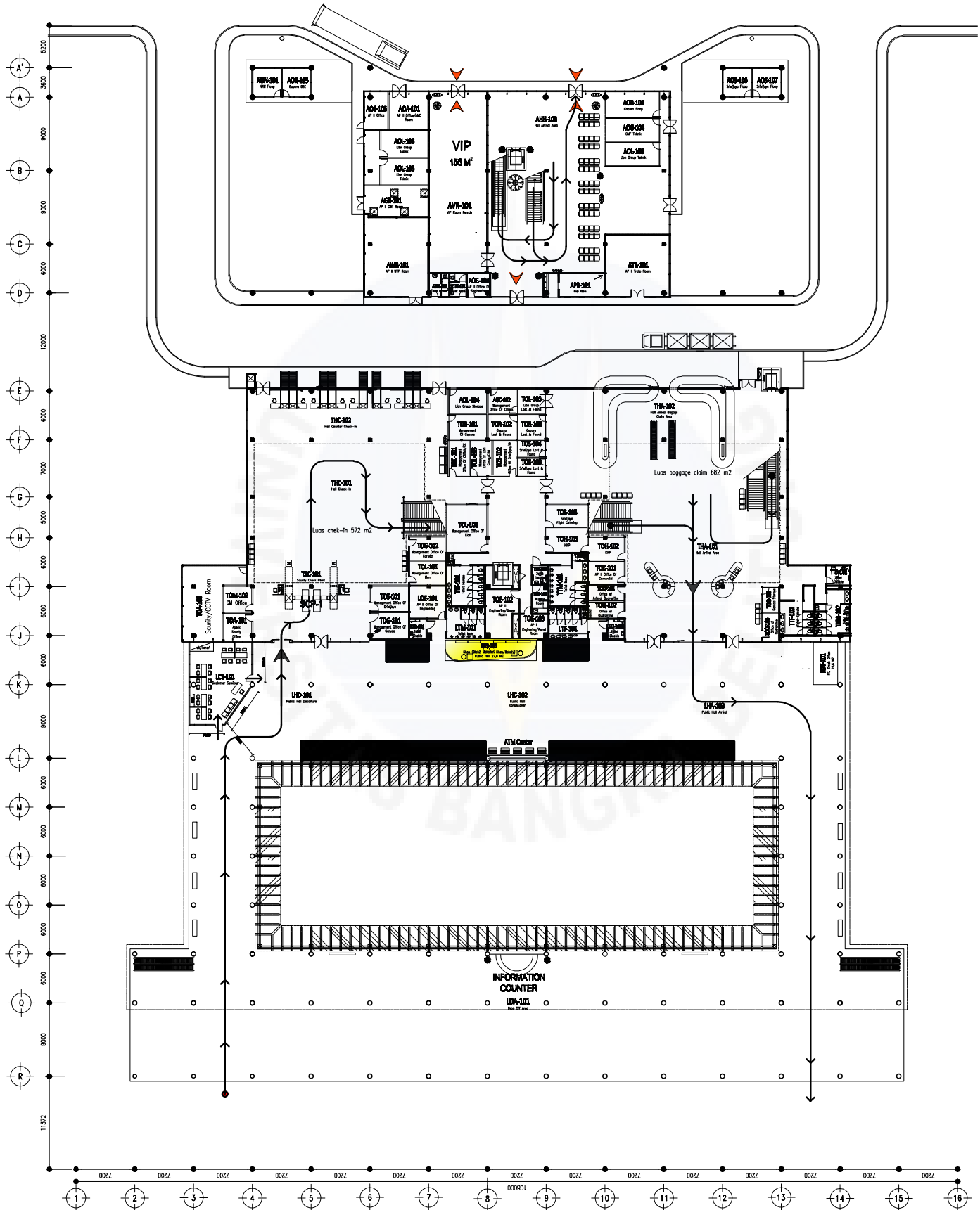
LAYOUT LANTAI 1
