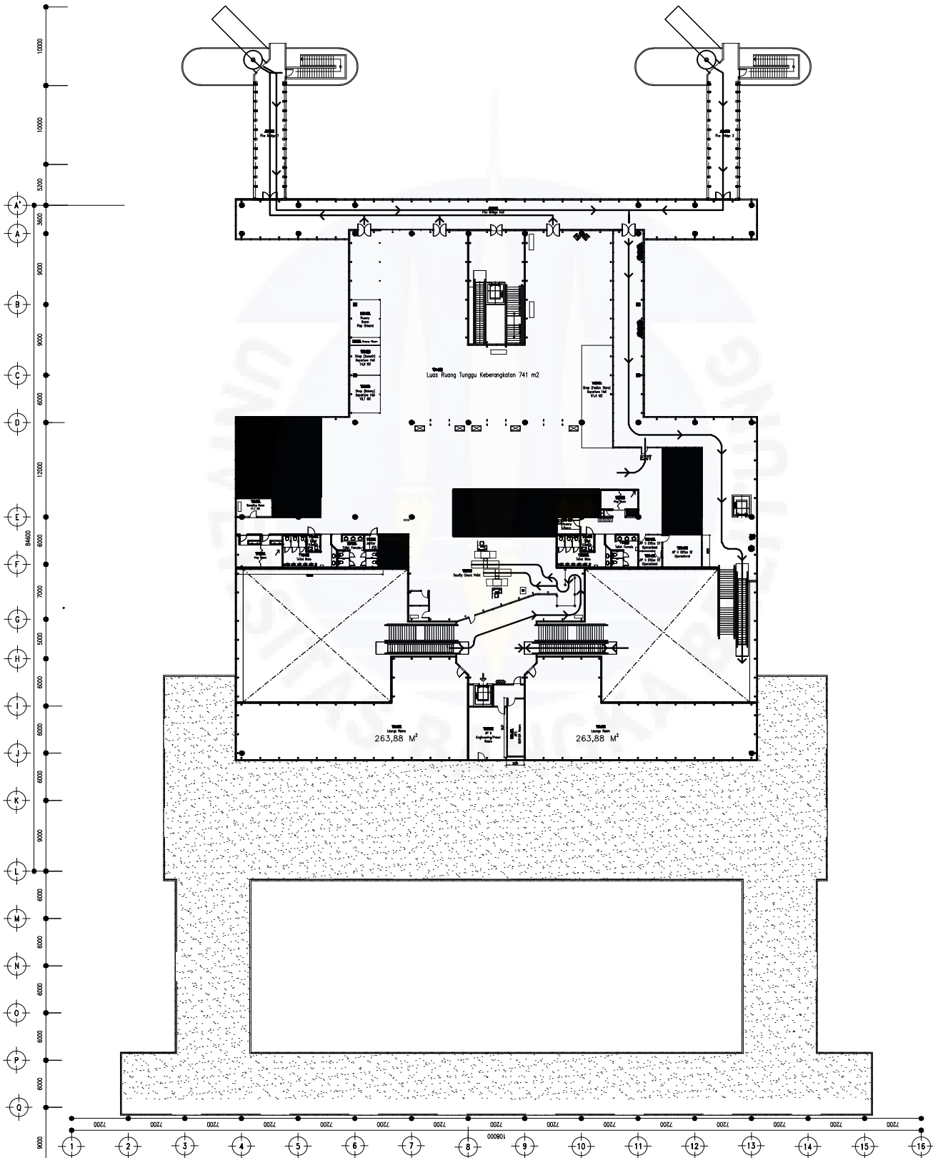
LAYOUT LANTAI 2
