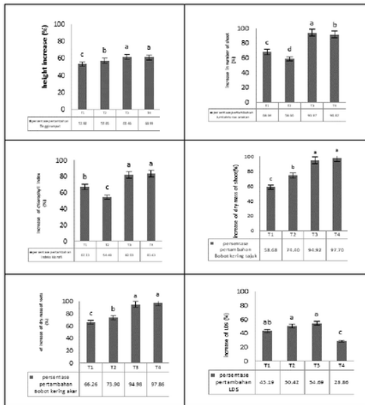
Fig. 1. The percentage (%) of increase of growth of the grass due to accumulation from t1, t2, t3,, and t4 as compared to control (t0) Notes: types of planting media: t1=tailings with addition of inorganic fertilizer NPK (15:15:15) 100kg/ha, t2=tailings with addition of organic matters 5% of total volume of tailings soil/polybag, t3=tailings with addition of lime+NPK (lime 6,8 ton /ha and 100kg NPK/ha), t4= tailings with addition of organic matter and inorganic fertilizer NPK ( composit of 5% of total volume of media/polybag) and NPK (100kg/ha). SAL= specific area of leaves, as compared to t0 (tailings with no additional treatment). Different alphabets in a graph and histogram shows significant differences of Duncan post-hoc test at 0.05. types of planting media: t1 = t2 = tailings soil with addition of inorganic fertilizer at 5% of the total volume of the tailings per polybag.
