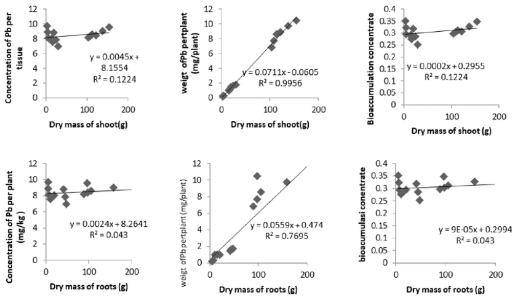
Fig. 2. The values of determination coefficient ( r^2 ) of grass dry mass and roots dry mass with concentration of Pb in the tissue (mg/kg), level of Pb in the plant (mg/plant) and bioaccumulation concentration of the hymenachne grass in tailings media
