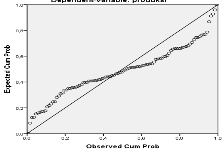
Normal P-P Plot of Regression Standardized Residual Dependent Variable: produksi
