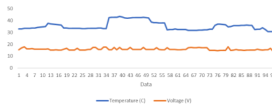
Figure 5. Voltage and Temperature from photovoltaic on July 23
