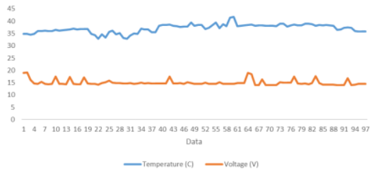
Figure 9. Voltage and Temperature from photovoltaic on July 25
