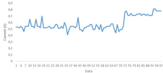
Figure 10. Current from photovoltaic on July 25
