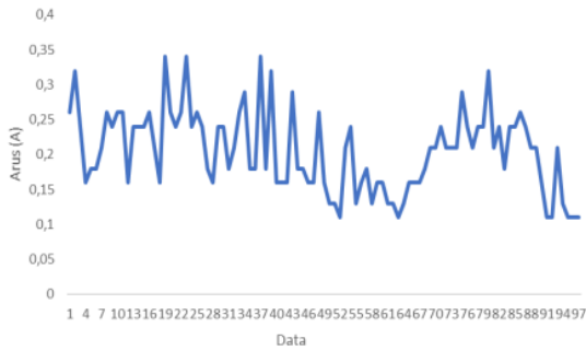
Figure 6. Current from photovoltaic on July 23
