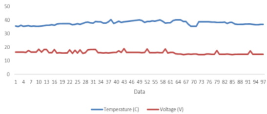
Figure 7. Voltage and Temperature from photovoltaic on July 24
