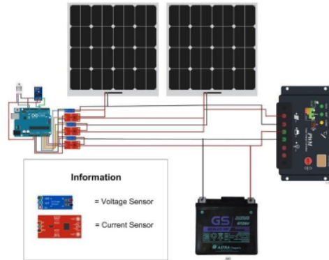
Figure 2. Circuit diagram
